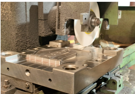
MOLD MACHINING
